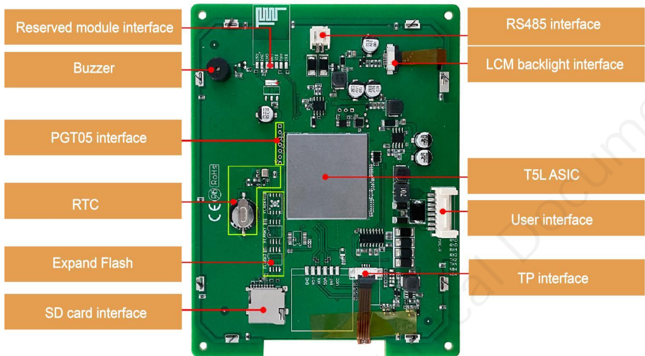
Hardware interface
