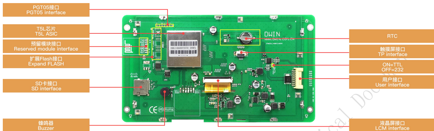
硬件接口图 Hardware interface
