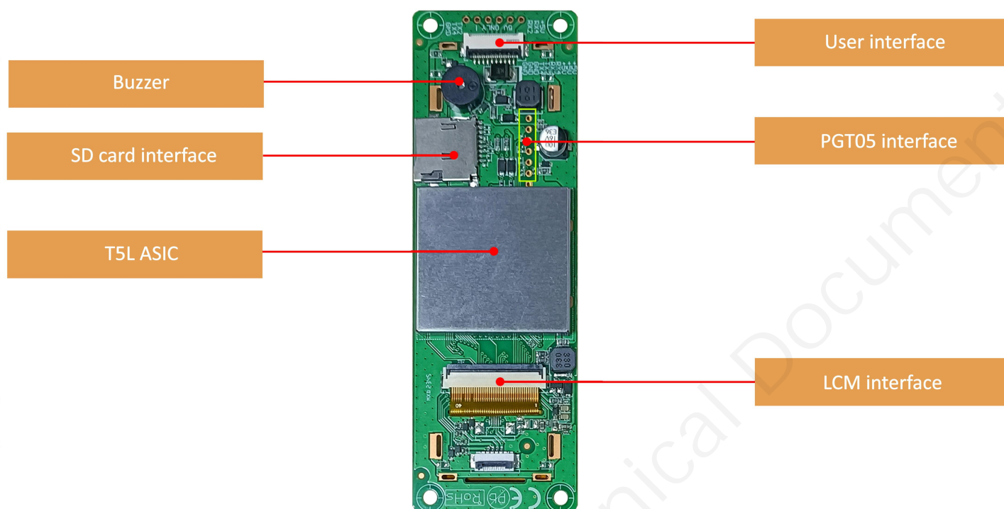
Hardware interface
