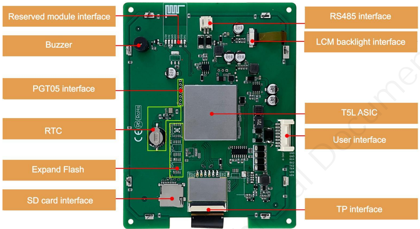
Hardware interface
